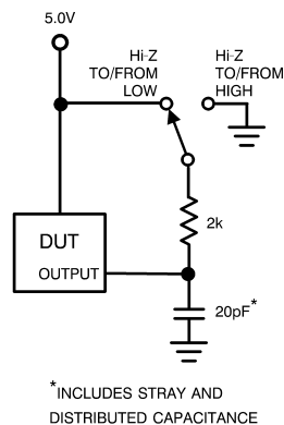
Figure 21. t_{EN} , t_{DIS} Test Circuit
